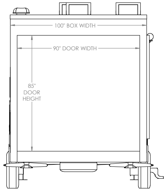
REAR
