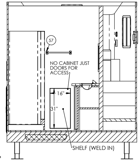
SECTION C-C INTERIOR FRONT
